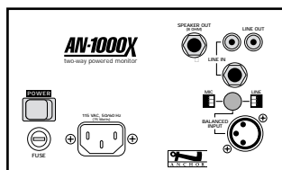
AN-1000X rear panel.
